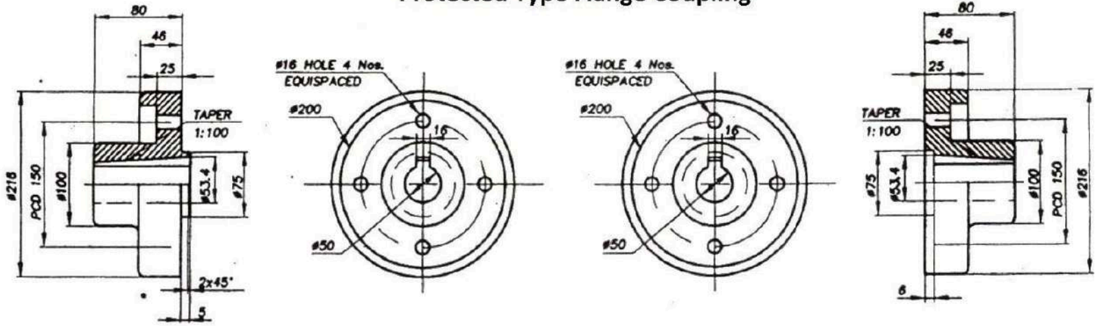
① FLANGE 1 MATL. C.I. QTY. = 2 Nos. ② FLANGE 2 MATL. C.I. QTY. = 2 Nos.
